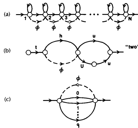
Fig. 8. Examples of networks incorporating null transitions. (a) Left-right model. (b) Finite state network. (c) Grammar network.
