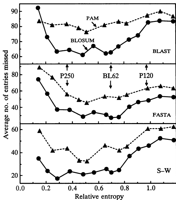
FIG. 3. Searching performance of programs using members of the guanine nucleotide-binding protein-coupled receptor family as queries and matrices from the BLOSUM and PAM series scaled in half-bits (11). Removal of this family from the BLOCKS data base led to a nearly identical matrix with similar performance. Matrices represented (left to right) are BLOSUM (BL) 30, 35, 40, 45, 50, 55, 60, 62, 65, 70, 75, 80, 85, and 90 and PAM (P) 400, 310, 250, 220, 200, 160, 150, 140, 120, 110, and 100. The average numbers of true positive Swiss-Prot entries missed are shown for LSHR$RAT, RTA$RAT, and UL33$HCMVA versus Swiss-Prot 20. Results using BLAST and FASTA or SSEARCH (S-W) are not comparable to each other, since different detection criteria were used for the three programs.
